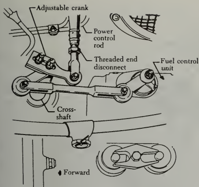
FIGURE 8-18. Power lever disconnect.
